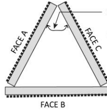
Signs with three or more sides and all angles greater than 45 degrees Sign area is computed as the sum of the area of the all faces. (Face A + Face B + Face C)
