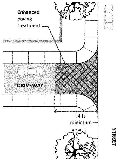
Figure 35-144B.7: Enhanced Paving For Entrance Driveways
