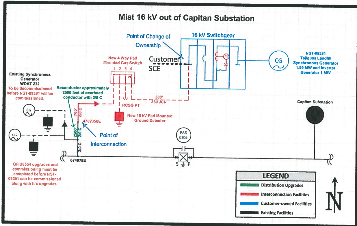
One-line Diagram Depicting the Generating Facility, Interconnection Facilities, Metering Equipment, and Upgrades
