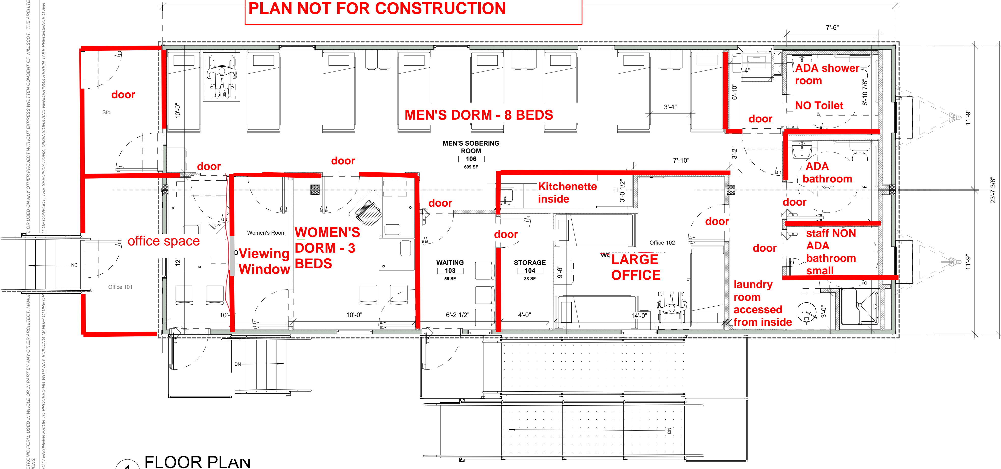
1 FLOOR PLAN
