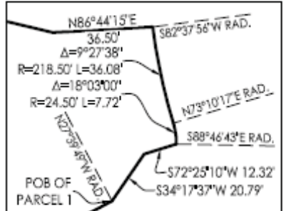
DETAIL A 1" = 40'
