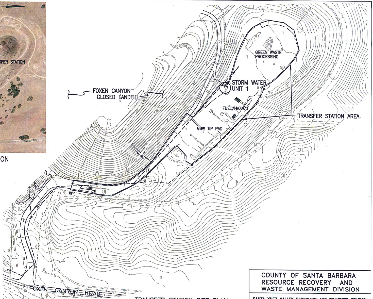
TRANSFER STATION SITE PLAN
