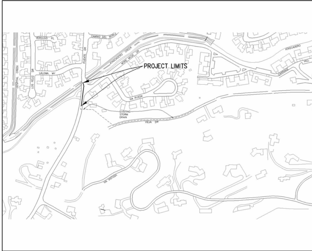
Via Rueda Storm Drain Interceptor II Project – Site Map
