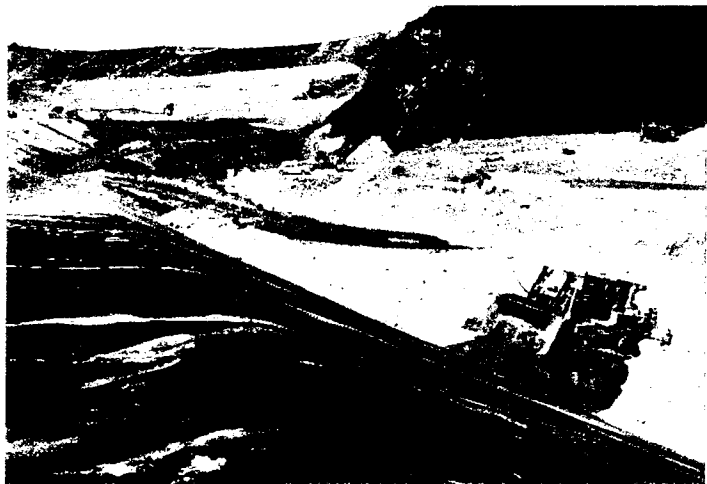
A dozer pushing protective cover soil up a lined slope at Tajiguas Landfill.
