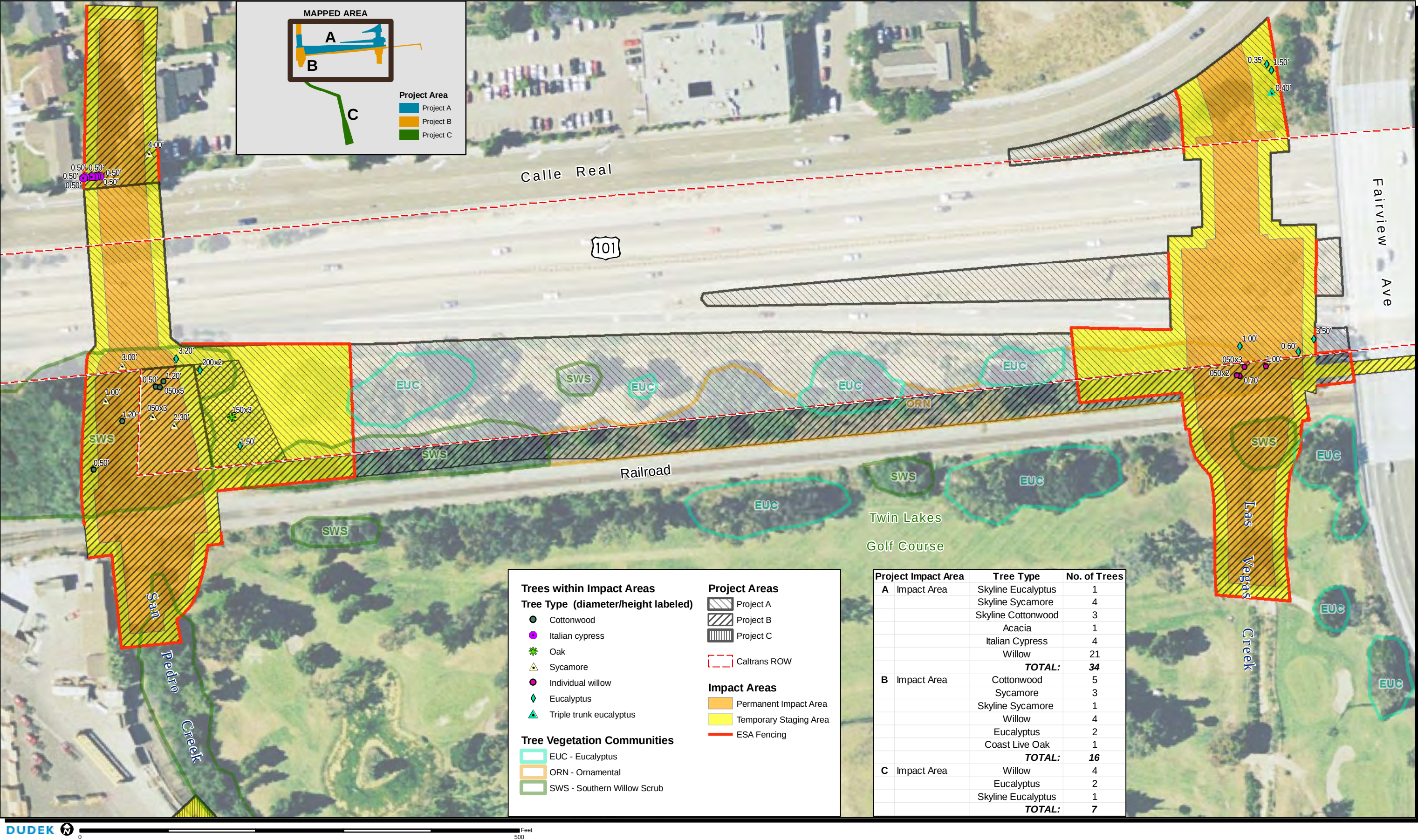
Las Vegas and San Pedro Creek Capacity Improvement Project Tree Protection/Removal Plan
