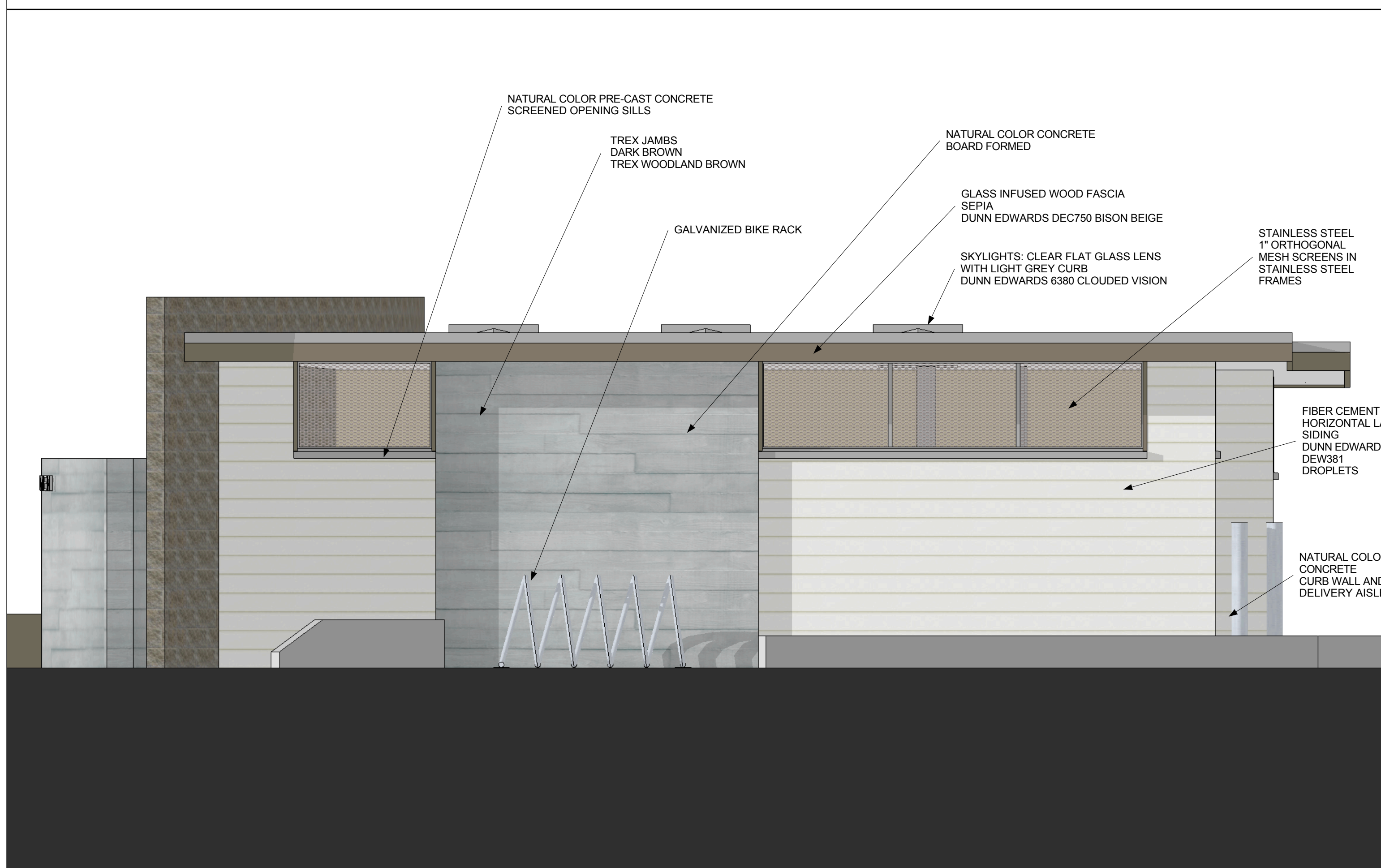
NORTH ELEVATION
