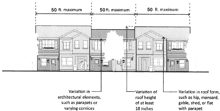
Figure 35.33-4
