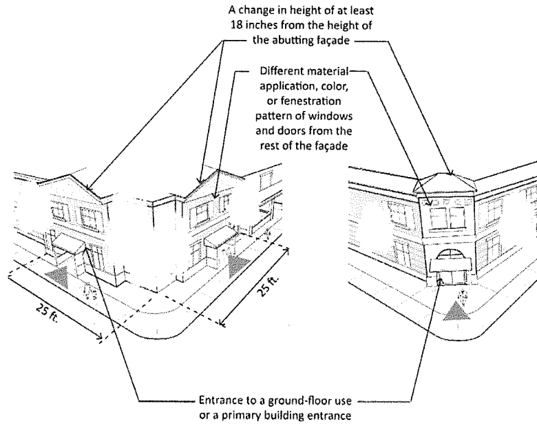
Figure 35.33-3: Corner Lots
