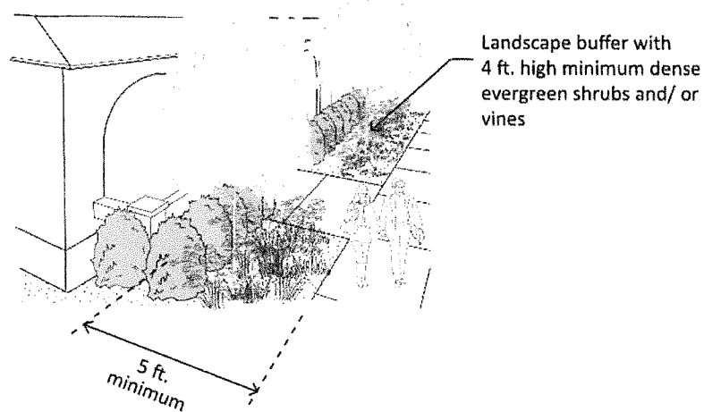
Figure 35.33-8: Landscape Buffer
