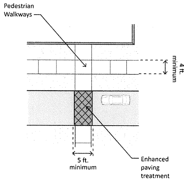
Figure 35.33-7: Pedestrian Walkways
