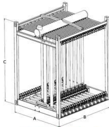
Figure 1: Drawing of 48M Cassette
