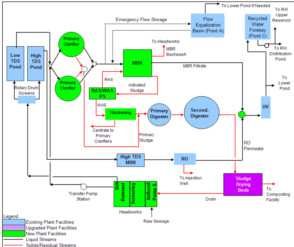
FIGURE 2-2 Proposed Phase I Process Flow Diagram and Plant Upgrades
