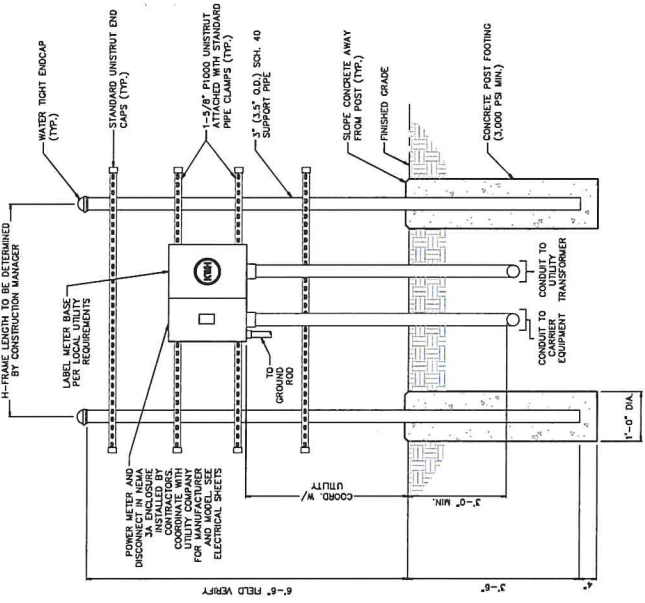
UTILITY H-FRAME DETAIL (METER SIDE) NOT TO SCALE
