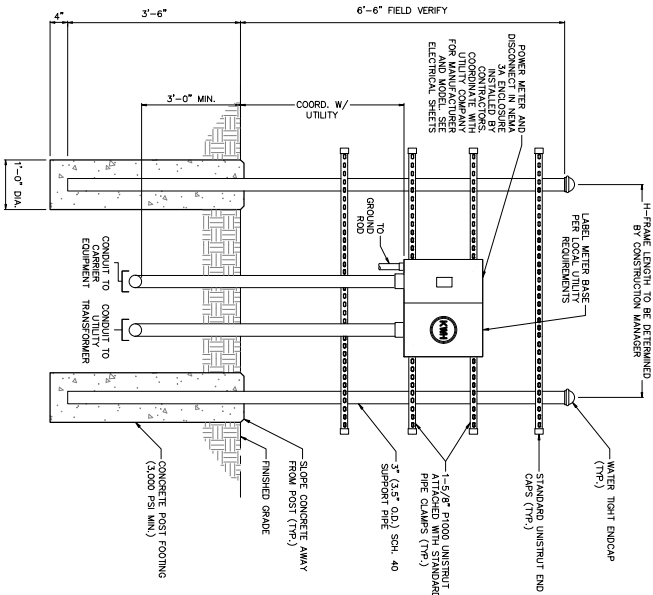
UTILITY H-FRAME DETAIL (METER SIDE) NOT TO SCALE
