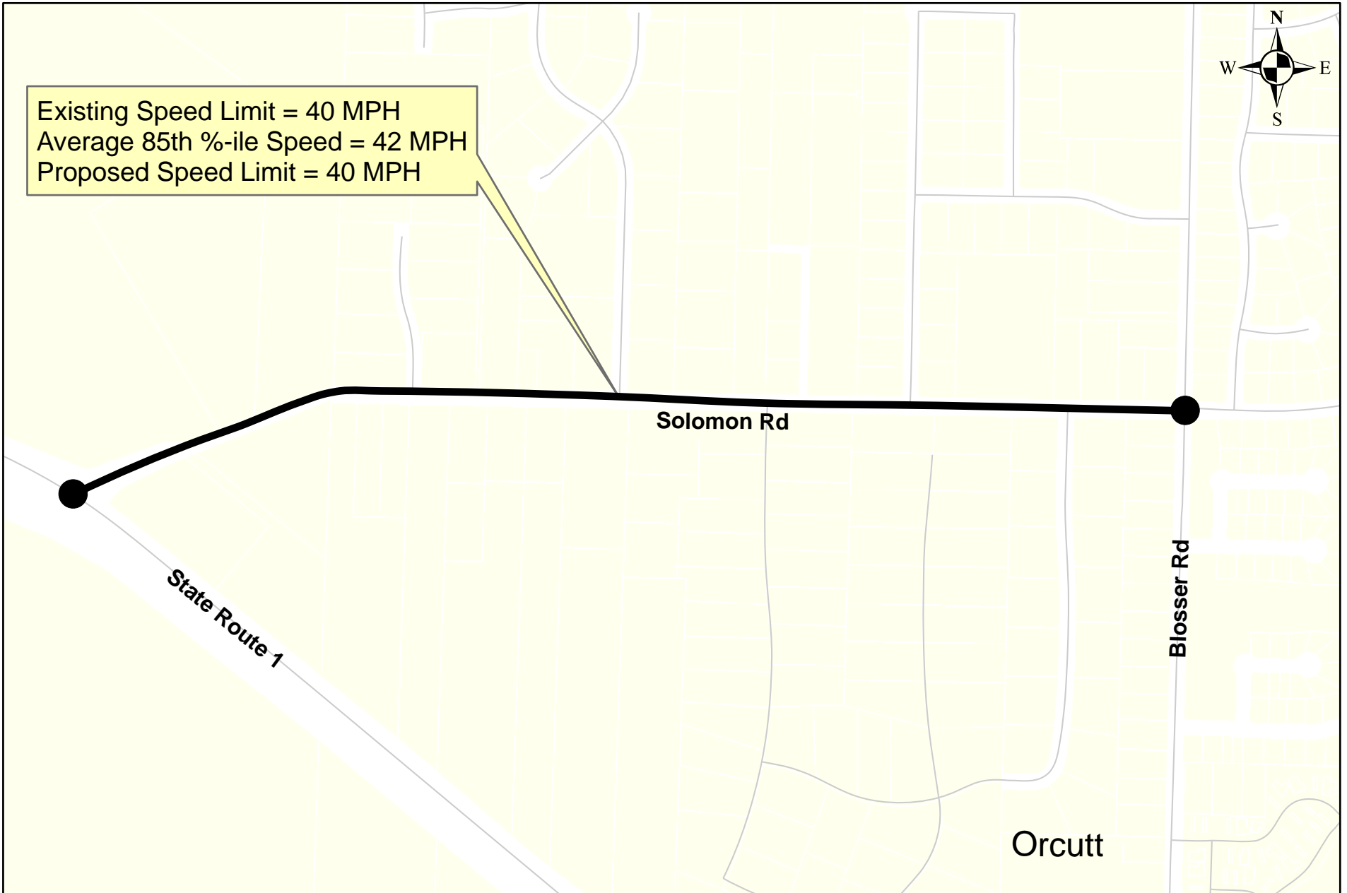
Proposed Speed Zone on Solomon Road (State Route 1 to Blosser Rd)
