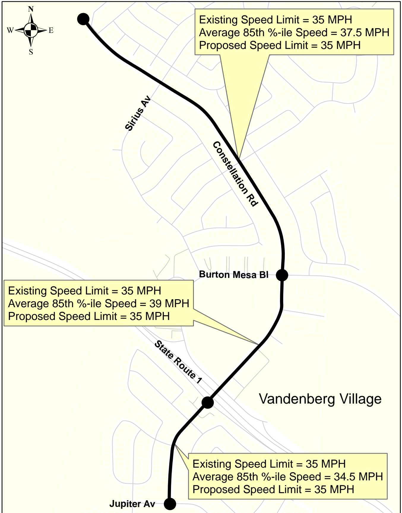
Proposed Speed Zone Constellation Road (Jupiter Av. to north end)
