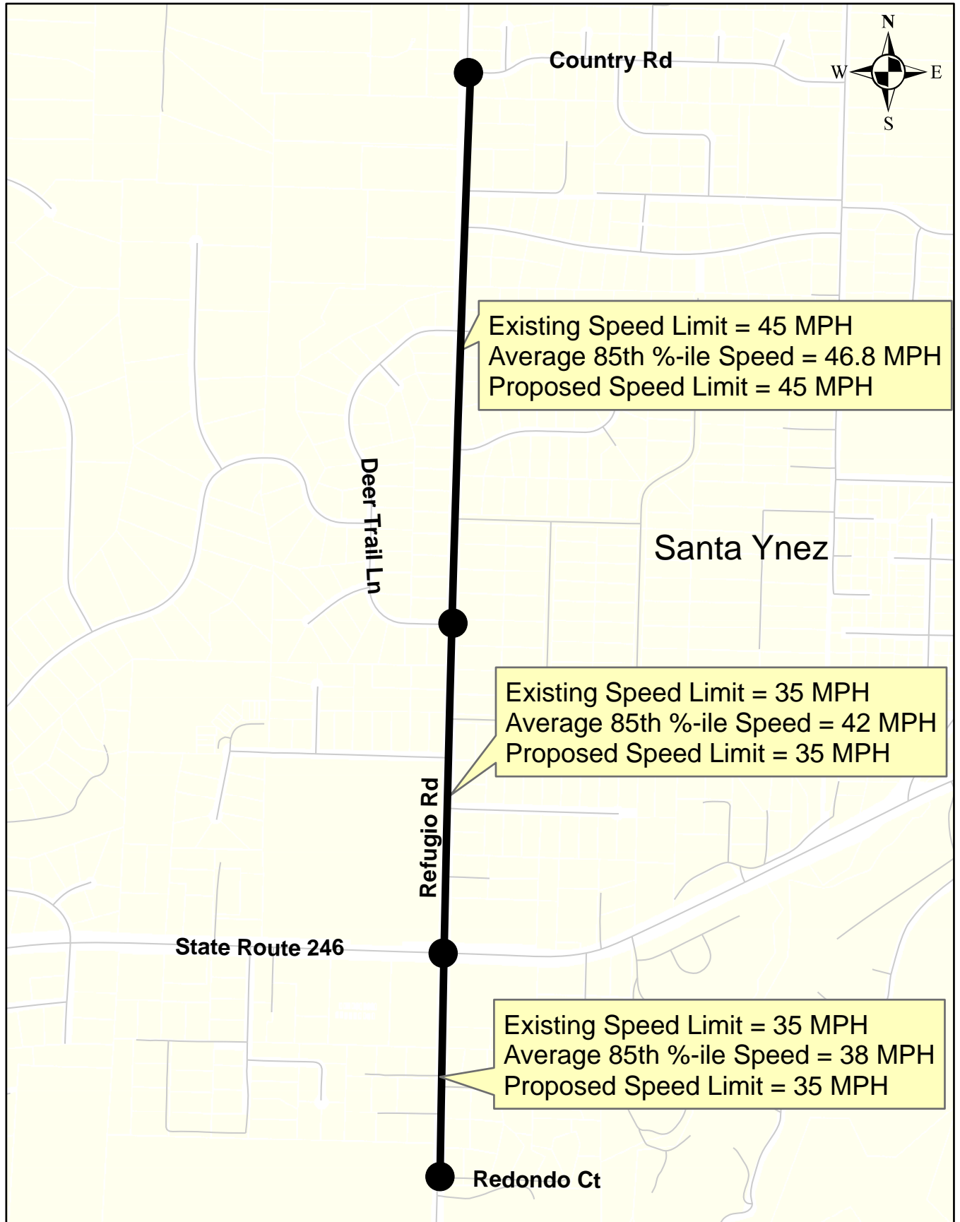
Proposed Speed Zone Refugio Road (Redondo Ct to Country Rd)
