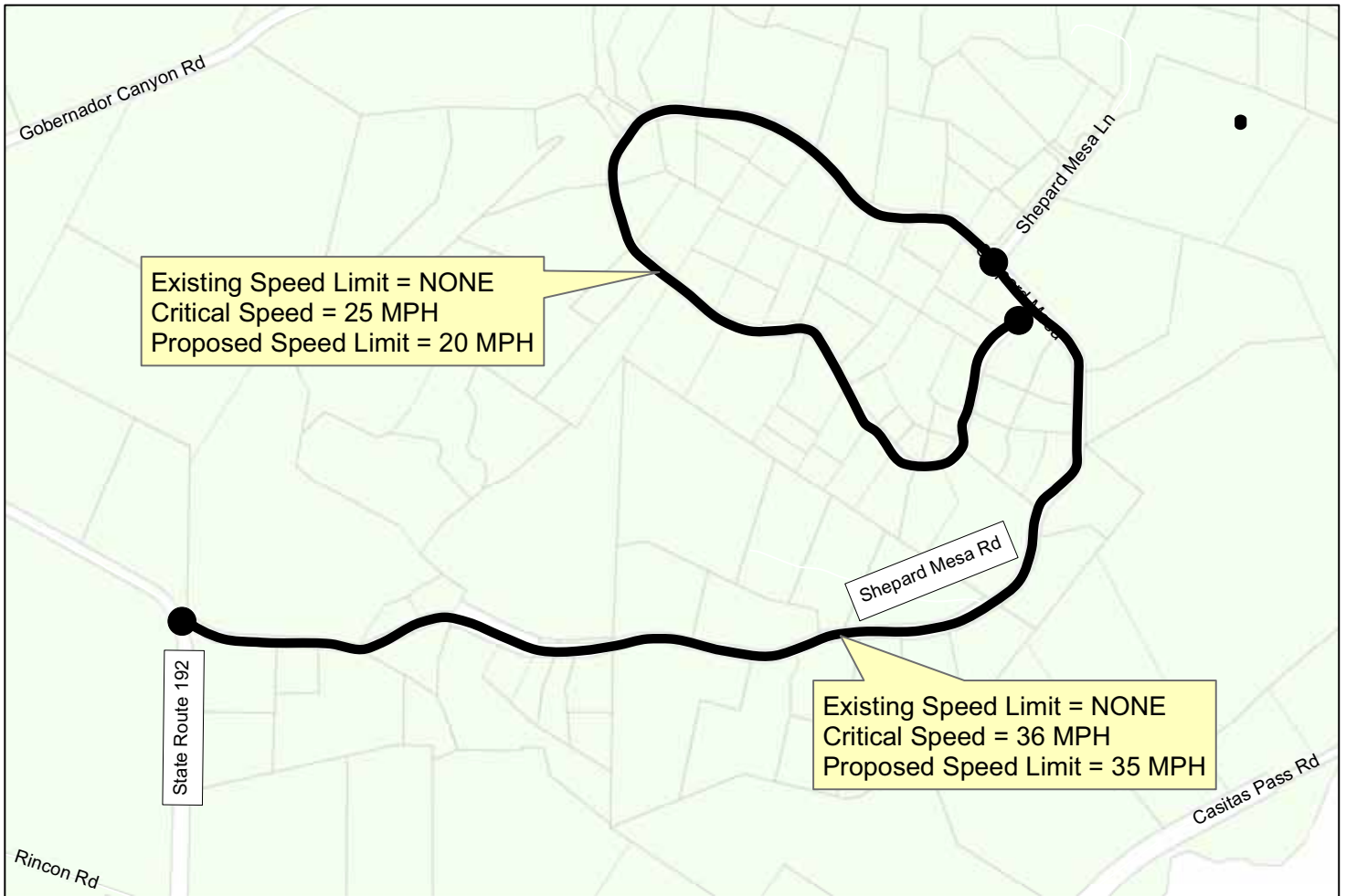
Proposed Speed Zone on Shepard Mesa Rd
