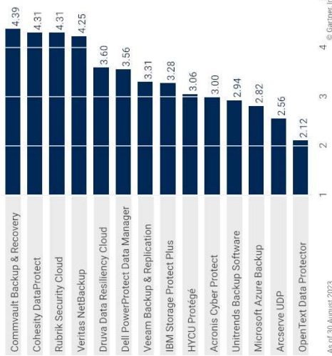
Product or Service Scores for Ransomware Detection, Protection and Recovery
