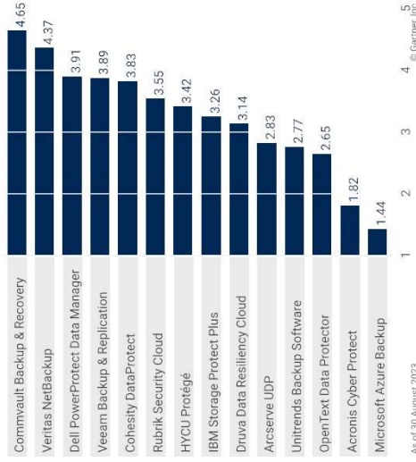
Product or Service Scores for Hybrid/Multicloud and SaaS
