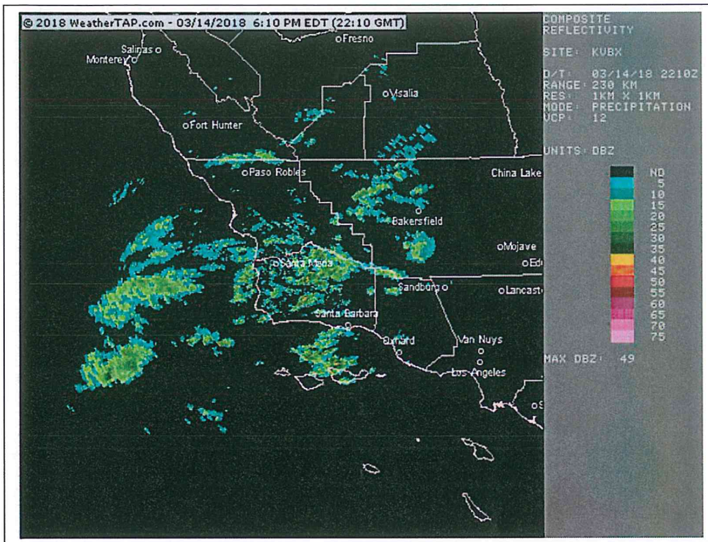
Figure 2.8 Vandenberg AFB NEXRAD Reflectivity, March 14, 2018 – Valid at 1510 PDT
