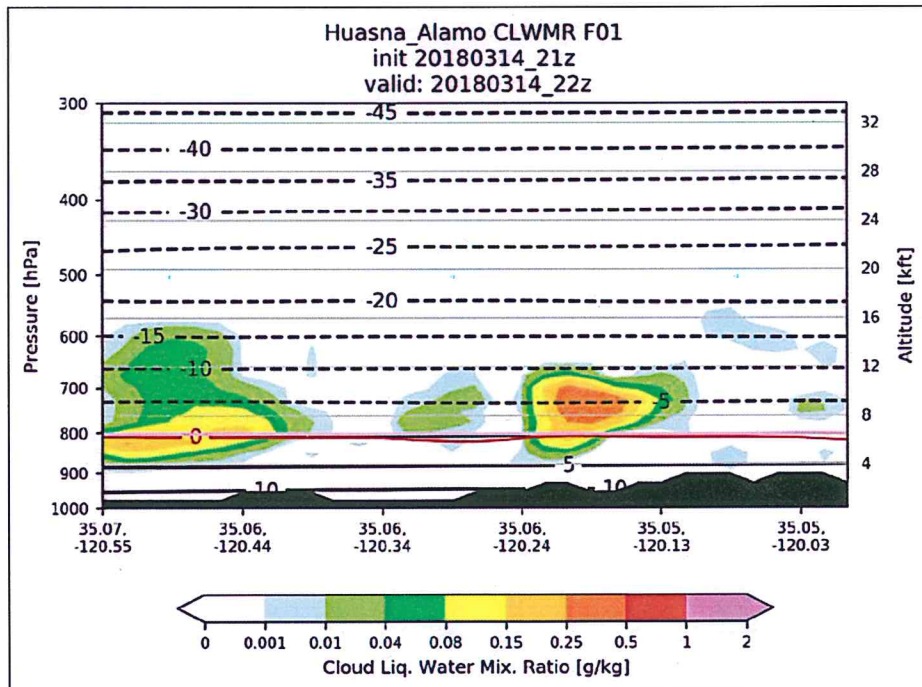
Figure 2.7 Cross Section of Liquid Water on March 14, 2018 – Valid at 1500 PDT
