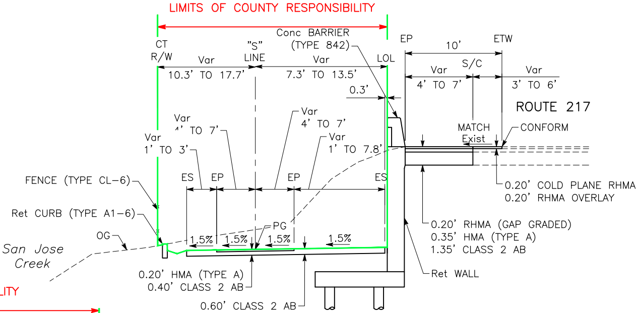
SECTION B-B NO SCALE
