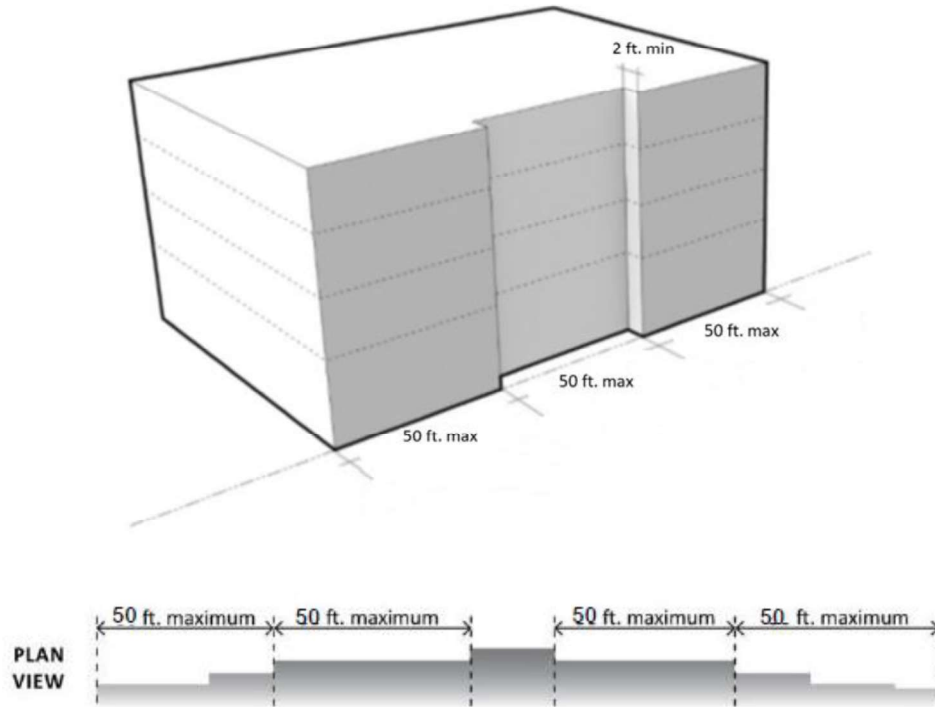
Figure 35.33-2 Wall Plane Variation
