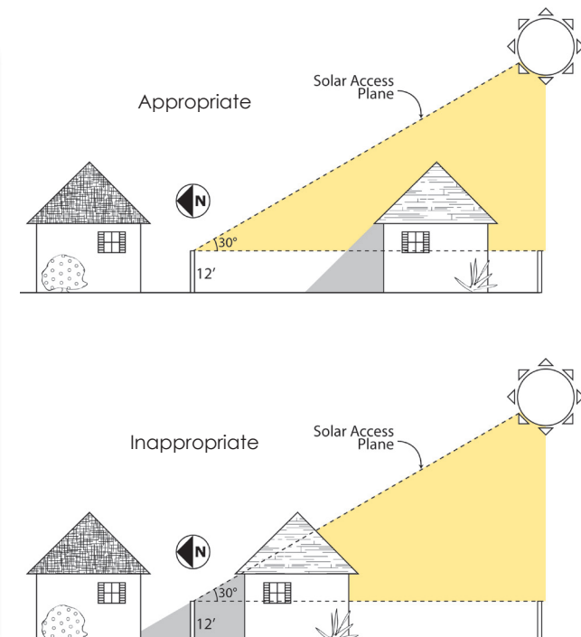
Figure 4.9 – Solar Access for structures near “northerly” property lines
