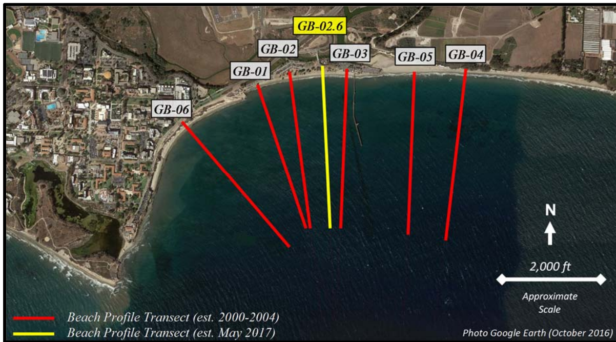
Figure 1. Goleta Beach Survey Transects
